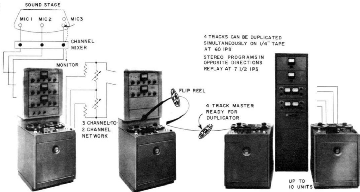
Fig. 407. The actual steps in preparing a master tape start with a multi-channel first master. This tape is then fed through a mixer to reduce the signals to two channels and recorded on a four-track tape. The new tape is flipped, two more channels dubbed on the other two tracks, and the new master is ready for duplication. (Ampex)
