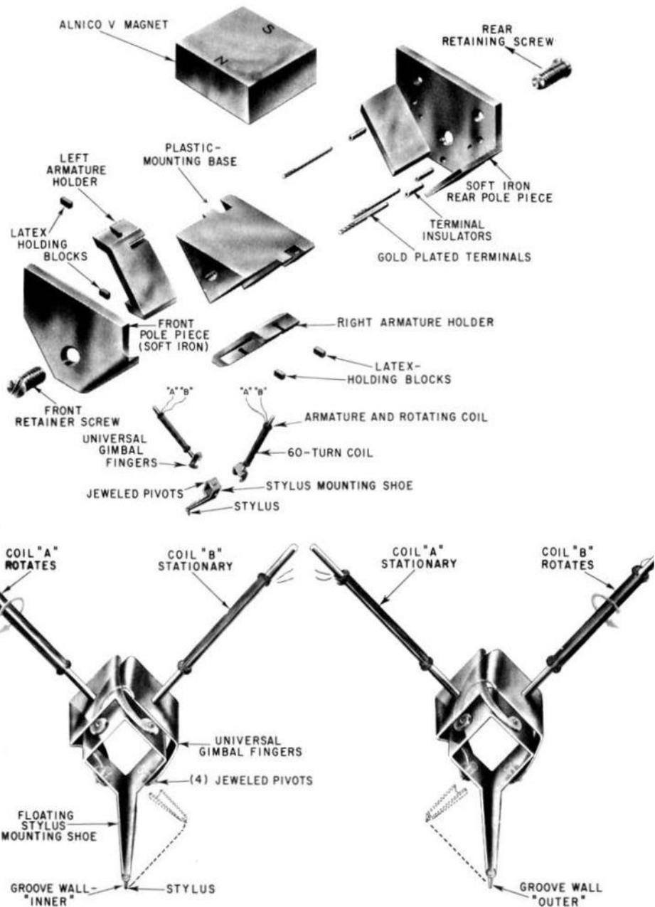
Fig. 509. (Top) Exploded view of magnetic stereo cartridge shows how the two independent rotating coils move in the field of a single Alnico magnet. Lower drawings show magnified detail of the stylus mounting and coil assemblies. Gimbal fingers allow maximum rotation in all directions resulting in high compliance.
